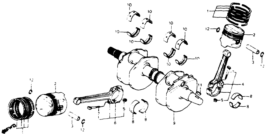
Crankshaft bearing selection (13300-MB0-010 ~ 2001586) (Oil clearance 28~52 μm)
